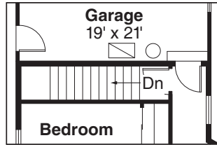
Alternate Basement Stairs
